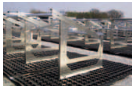
Vertically adjustable Solar Base Frames and Adapter Profiles for levelling out roof pitch and installation of large modules.
