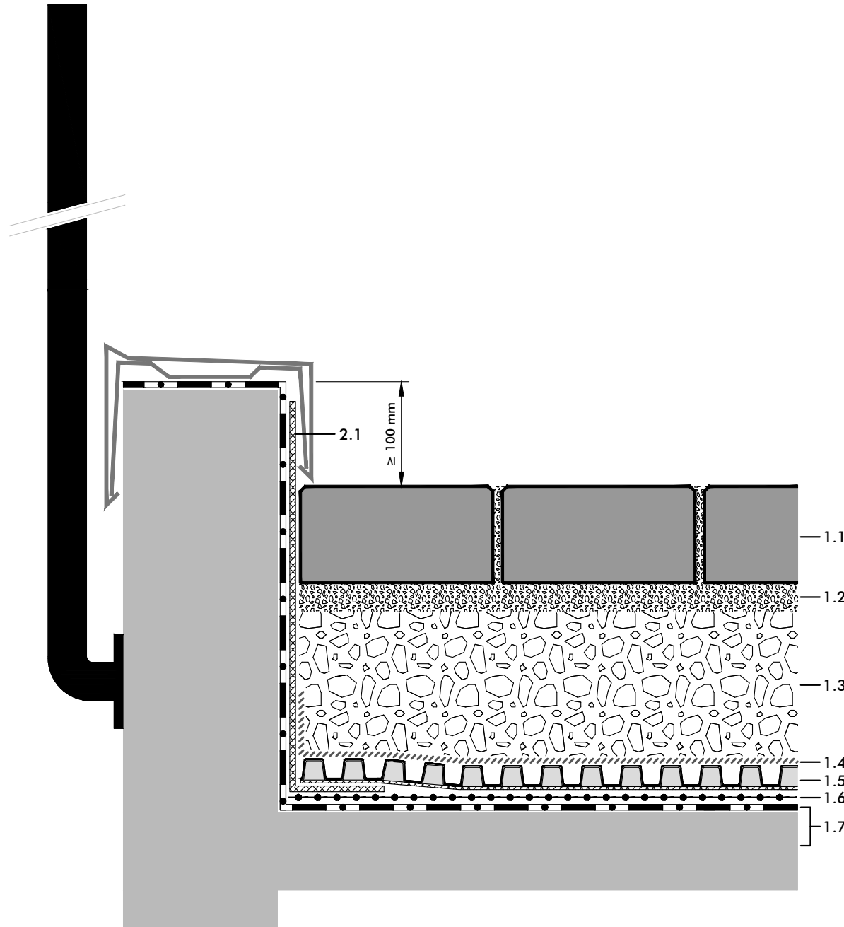
2.1 Protection Mat Strip SM-R
