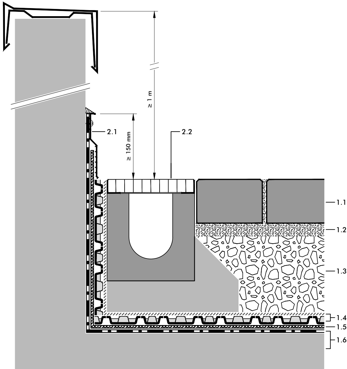
2.1 Clamping and Protection Profile AP 150 2.2 Concrete channel in concrete foundation
