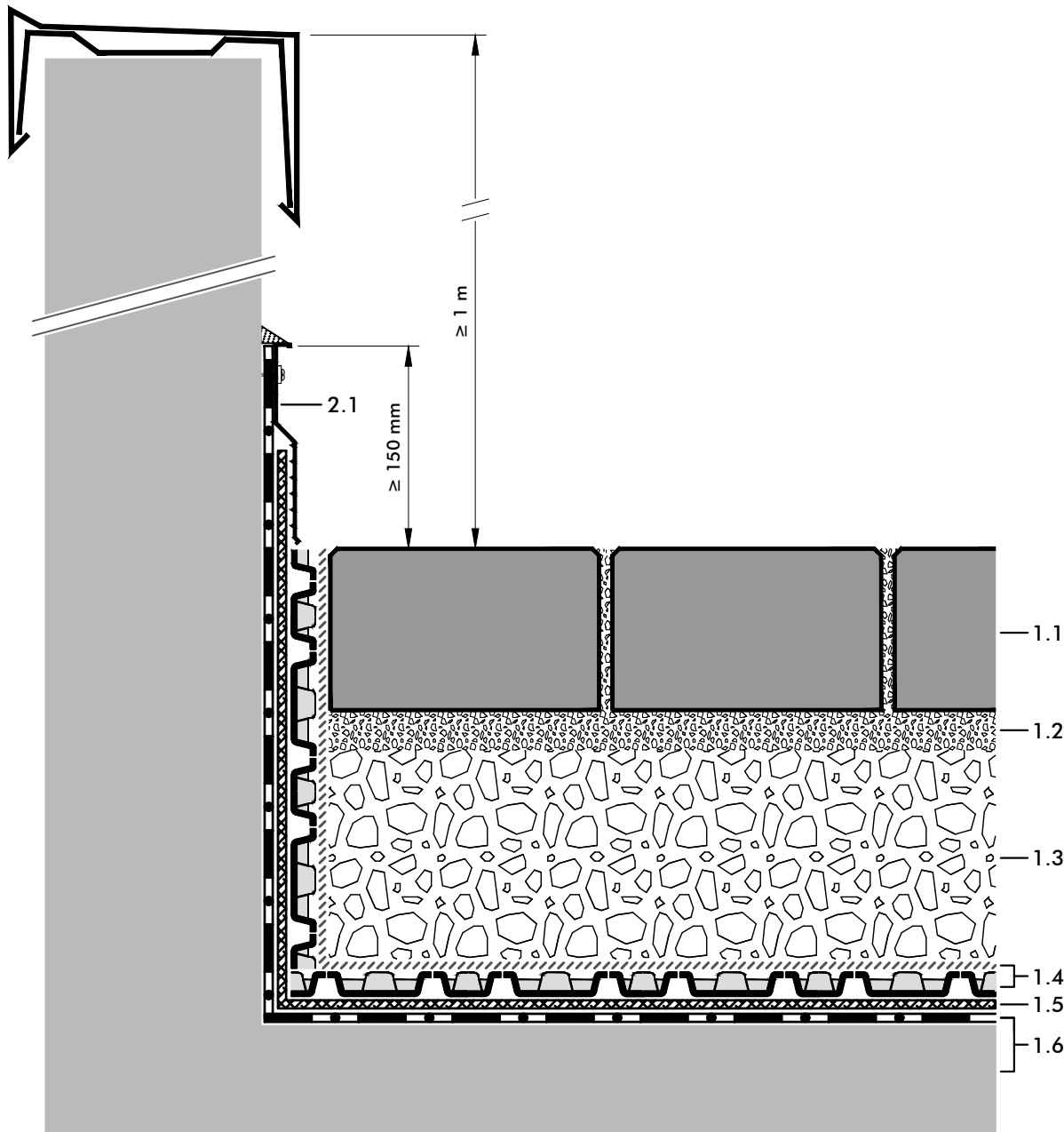
2.1 Clamping and Protection Profile AP 150
